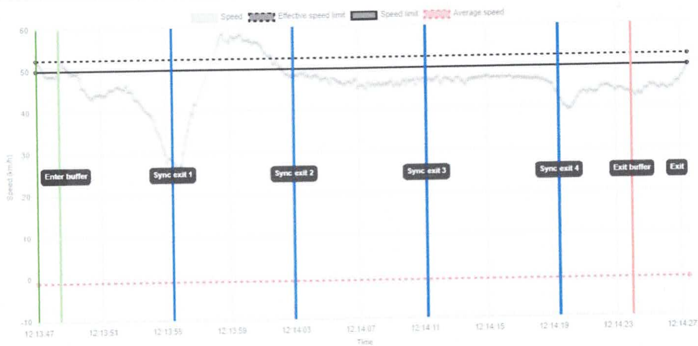
Speed graph over "SZ PS3-6 Montevaso" for "087"
